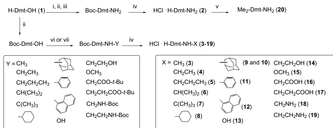
Scheme 1. Synthetic scheme for the Dmt compound library. Reagents and conditions: (i) SOCl 2 /CH 3 OH; (ii) (Boc) 2 O and Et 3 N; (iii) NH 3 /CH 3 OH; (iv) HCl/dioxane; (v) HCHO and NaBH 3 CN; (vi) PyBop, N,N -diisopropylethylamine and NH 2 -Y; (vii) isobutyl chloroformate, Et 3 N, and NH 2 -Y.
